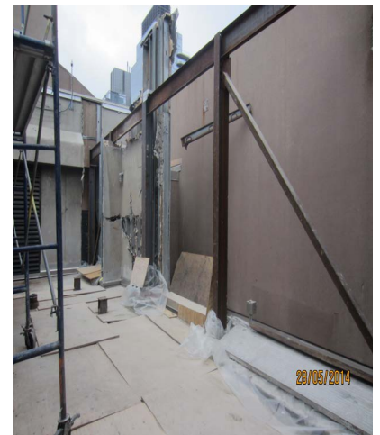
EIFS wall removal on roof.
